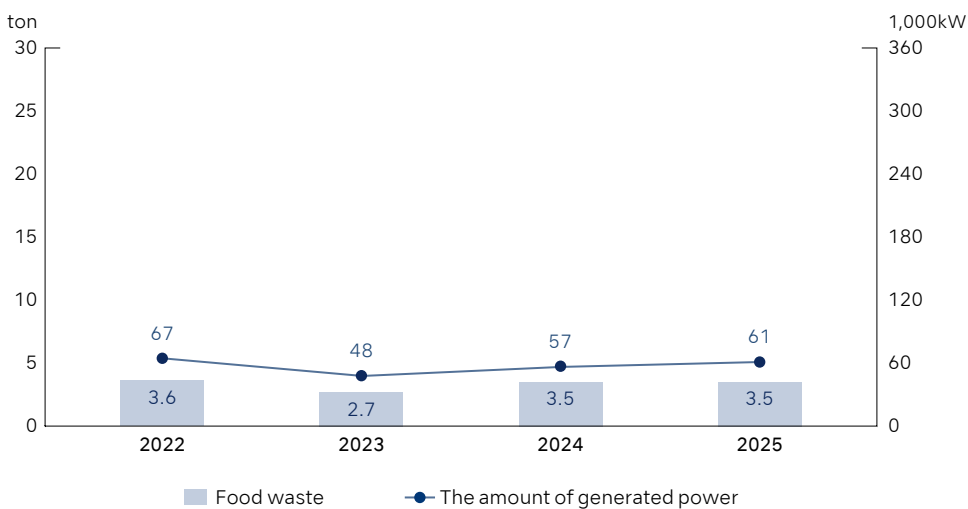
Relationships between food waste and the amount of generated power
